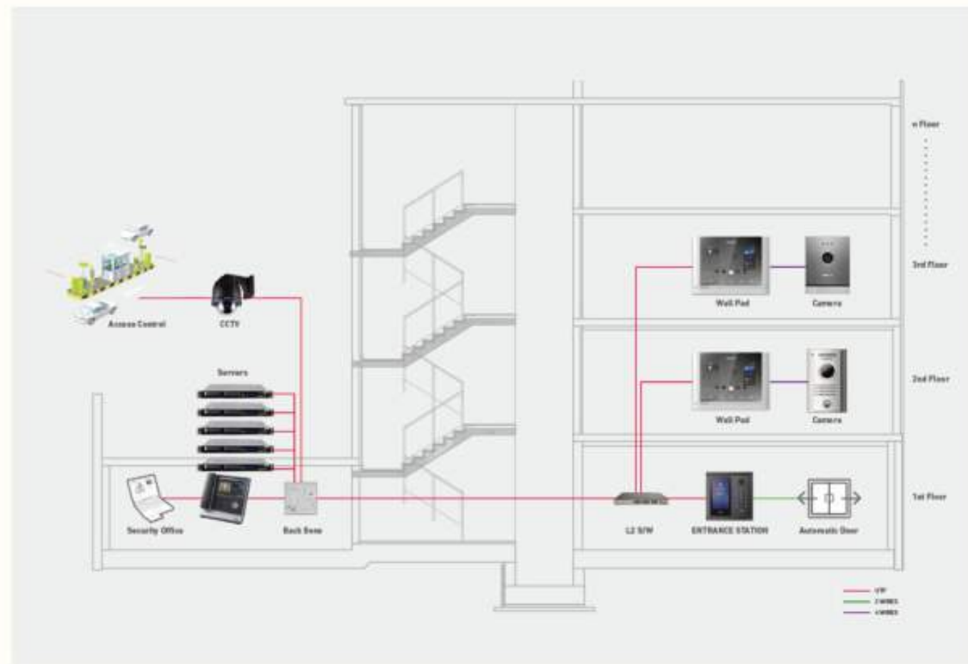
FIELD OF IP VIDEO PHONE SYSTEM APPLICATION
