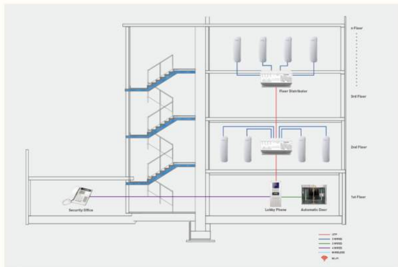
FIELD OF AUDIO GATE SYSTEM APPLICATION
